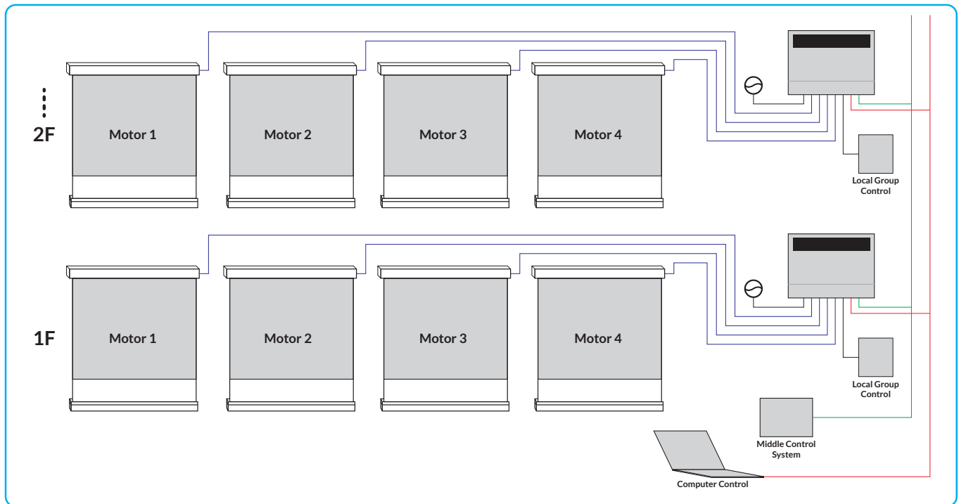
Application Mode Diagram
