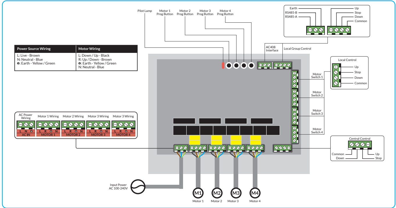
Controller Wiring Diagram
